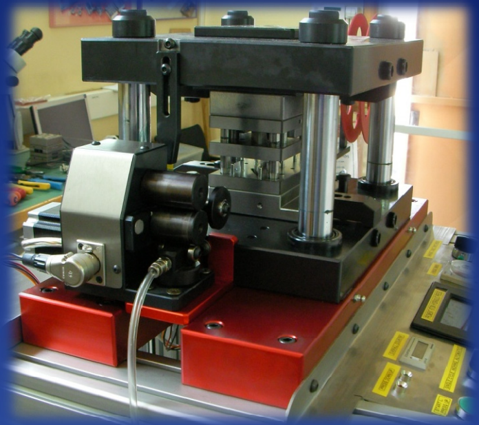
Proment 8 ton press with integral digital feeder and Master Die Set.
