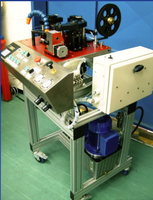
Fully Automated Soldering Machine
